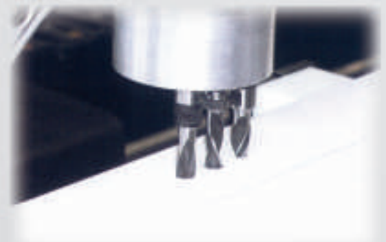
Drills for triple-drill units with male thread or cylindric plain shank
